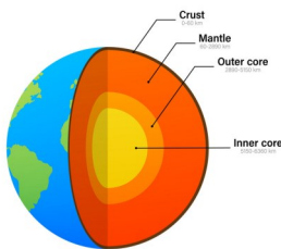
STRUCTURE OF THE EARTH
